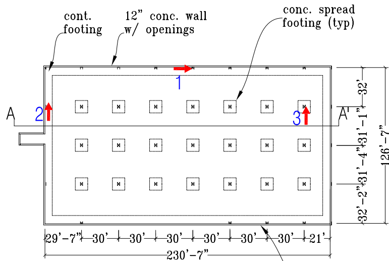
Basement
