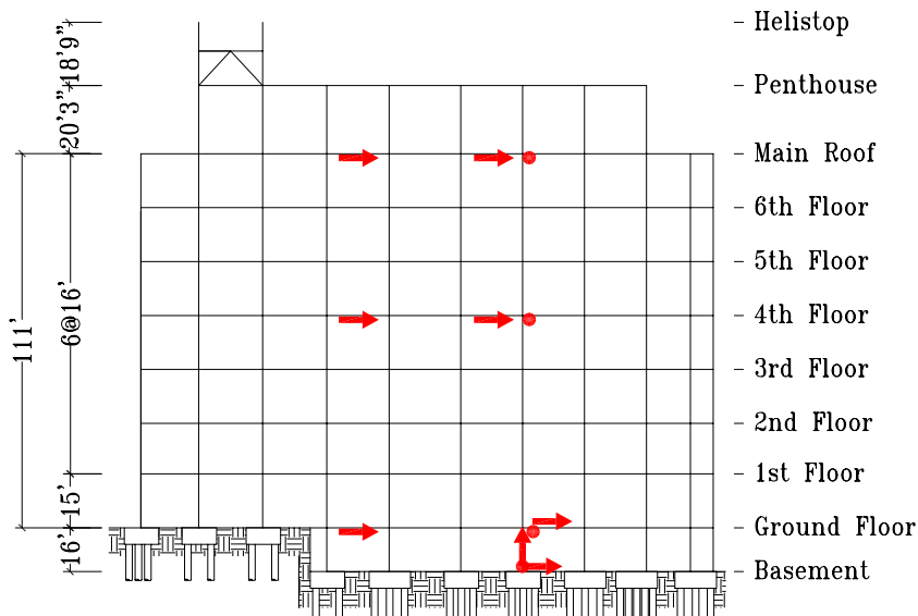
E/W Section
