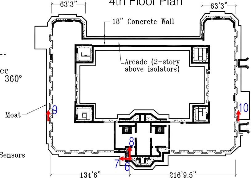
Basement (above isolators) Plan
