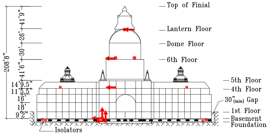
N/S Section
