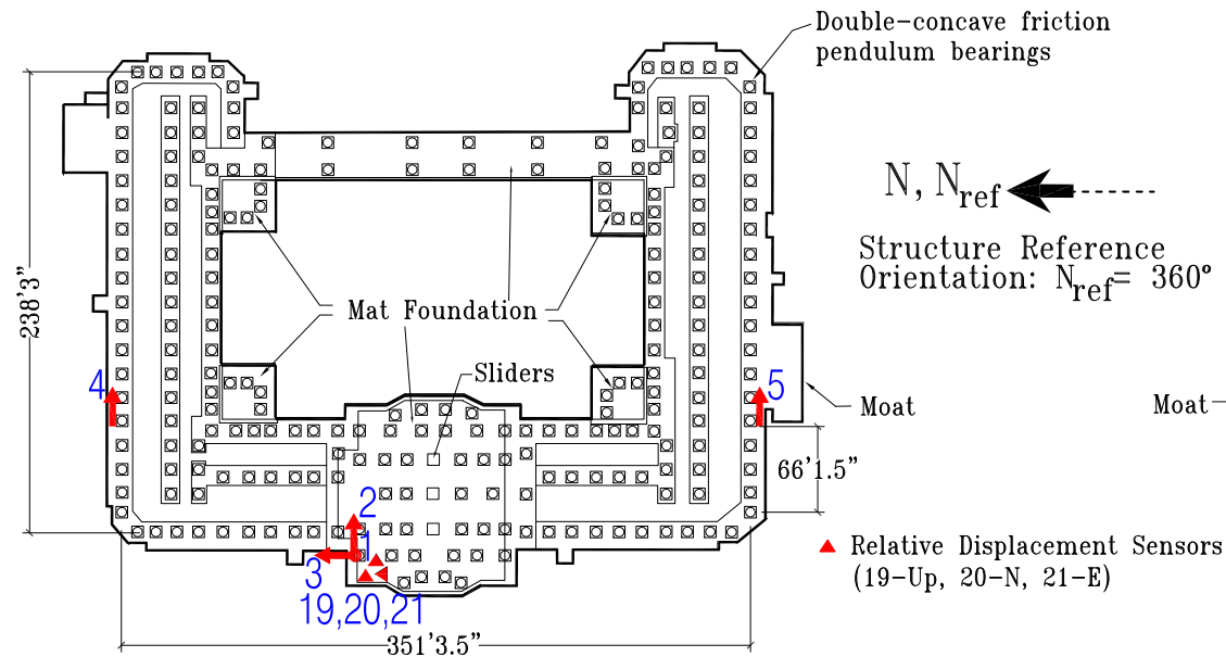
Foundation (below isolators) Plan
