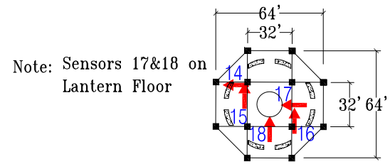
6th Floor Plan
