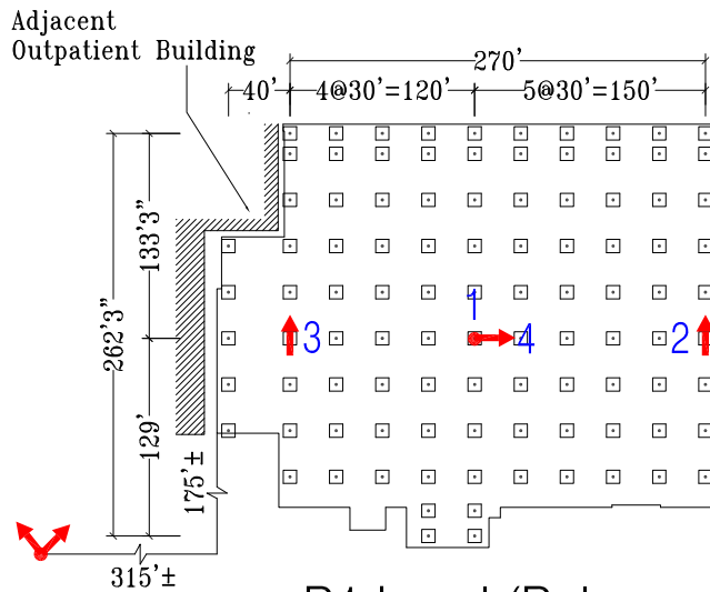
B1 Level (Below Isolators) Plan
