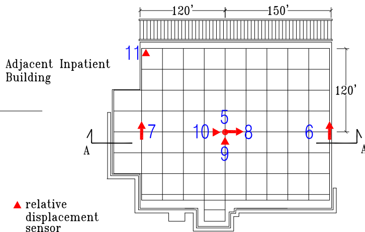
1st Level (Above Isolators) Plan
