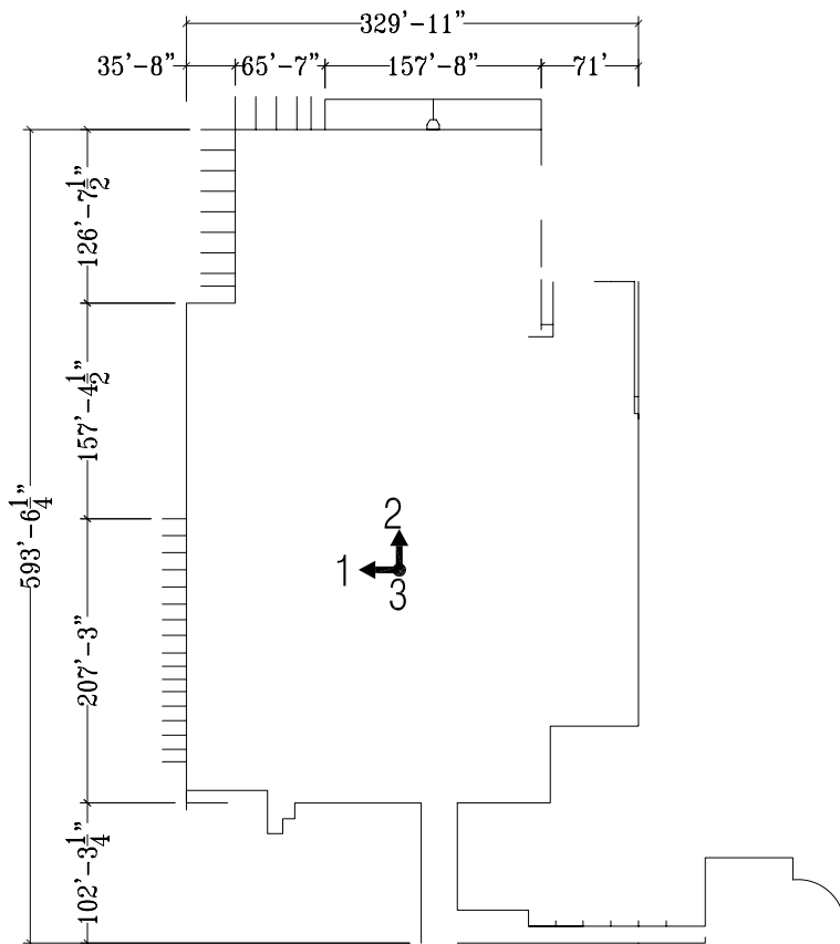
1st Level Plan
