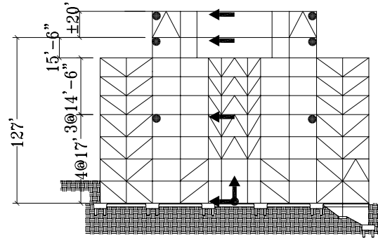
N/S Section
