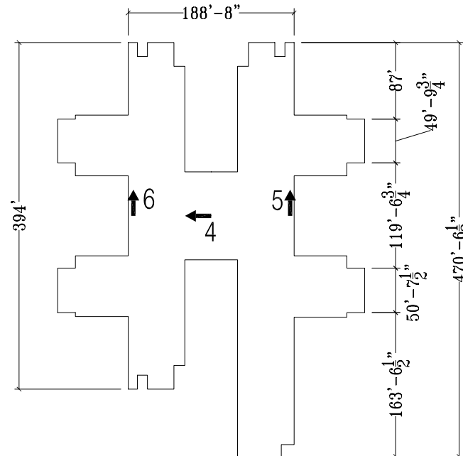
5th Level Plan
