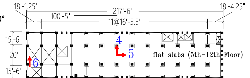
8th Floor Plan
