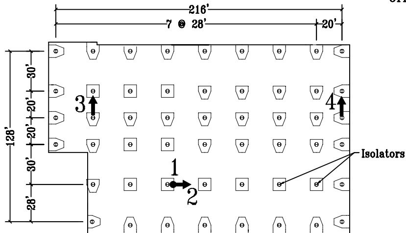
Foundation Plan
