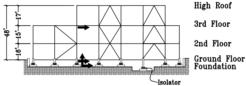
Elevation (East)
