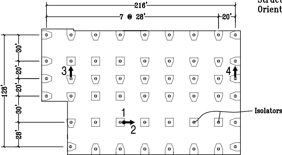
Foundation Plan
