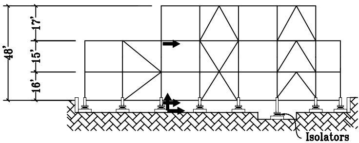
Elevation (South)
