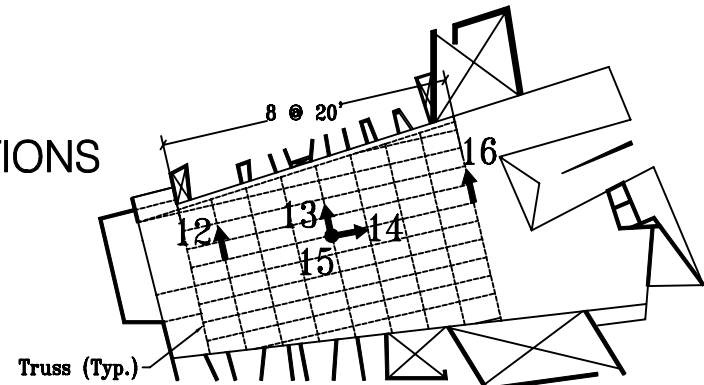
Roof Level Plan
