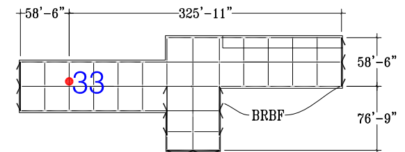
Level 16 Plan
