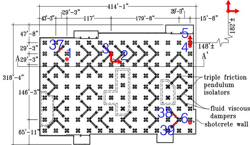
Level B/Foundation Plan (Below Isolators)
