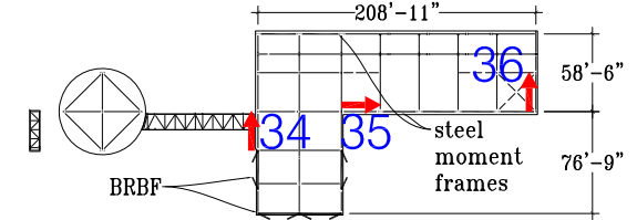
Level 17/Roof Plan
