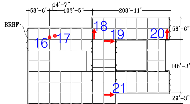
Level 6 Plan
