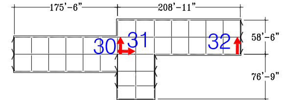
Level 13 Plan
