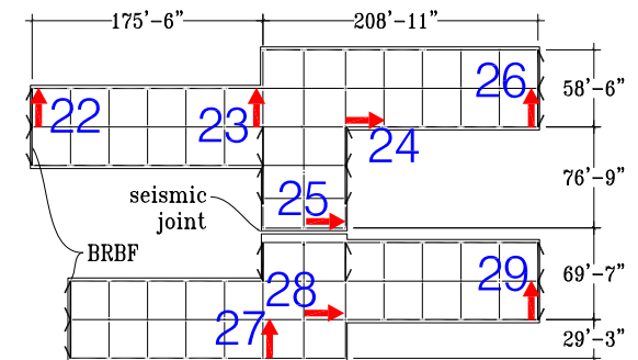
Level 10 Plan
