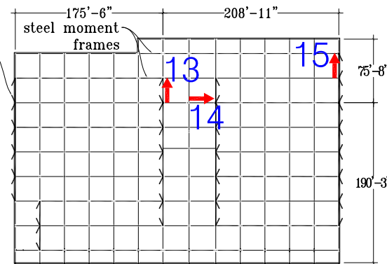
Level 4 Plan
