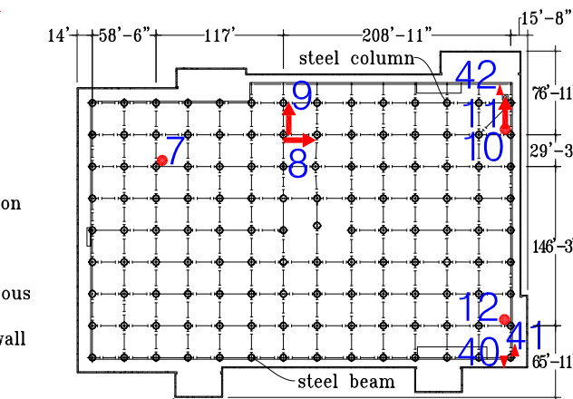
Level A Plan (Above Isolators)
