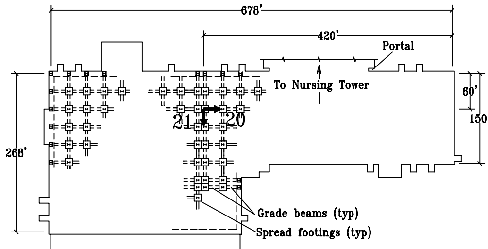
Foundation Plan (below isolators)
