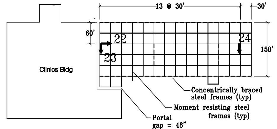
Ground Floor Plan (above isolators)
