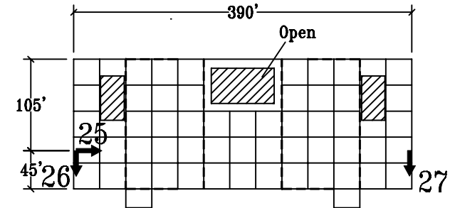
Roof Plan
