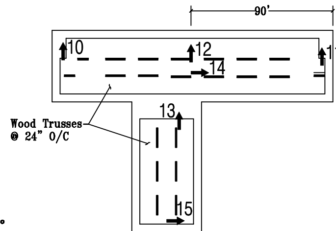
Roof Plan
