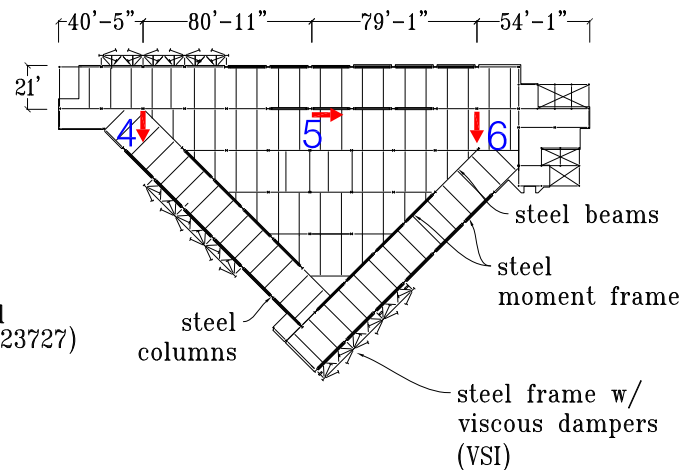
Level 2 Plan
