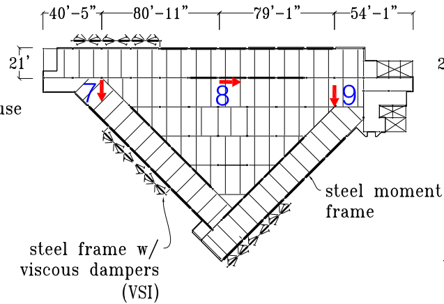
Level 4 Plan
