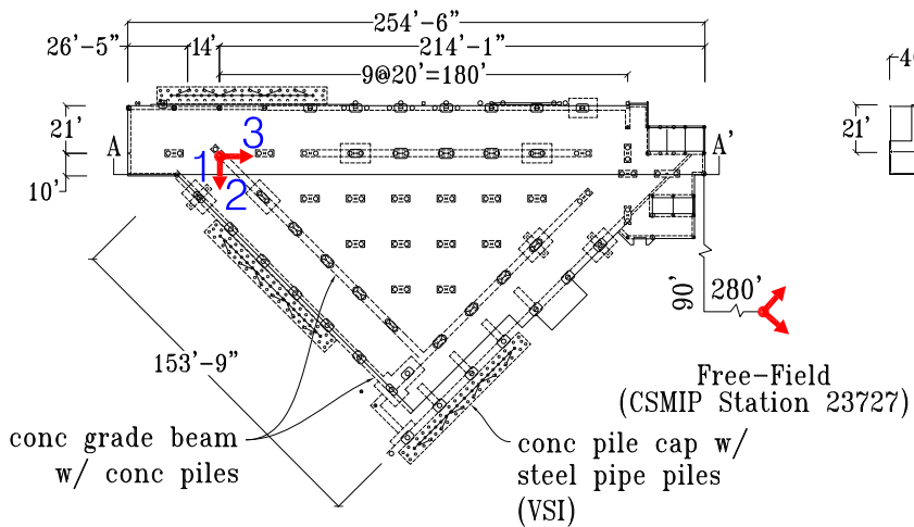
Level 1/Foundation Plan
