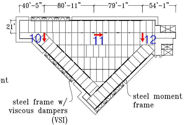
Roof Plan
