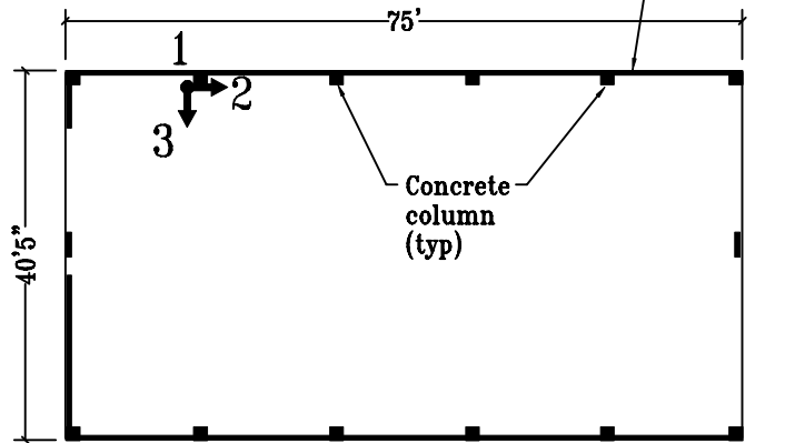
Ground Level Plan
