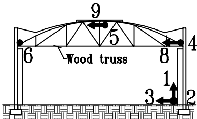
Building Section
