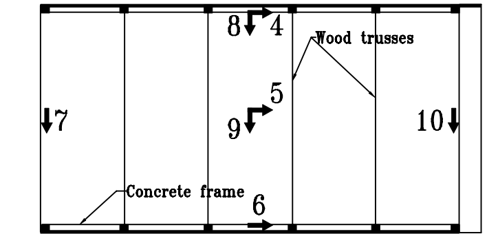
Roof Plan
