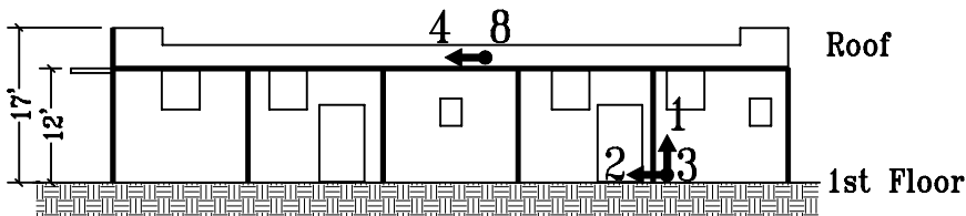
North Wall
