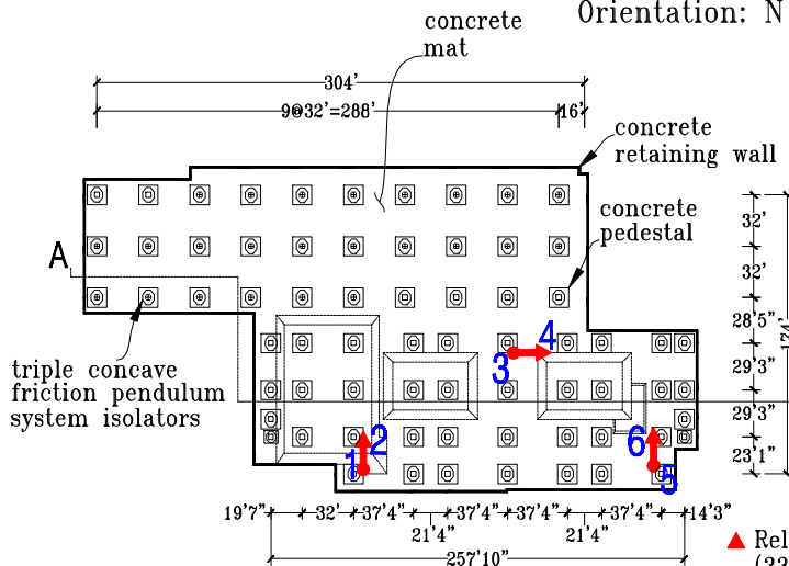
Foundation (Below Isolator) Plan
