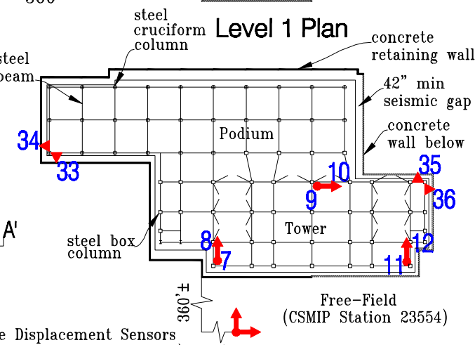
Lower Level (Above Isolator) Plan
