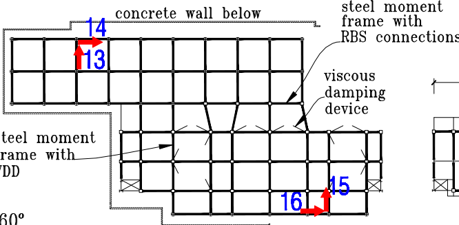
Level 1 Plan
