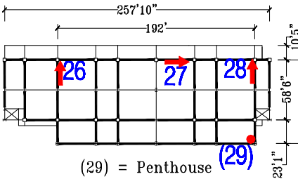
Level 11 Plan
