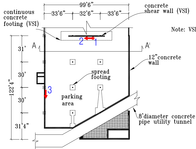
Basement Plan
