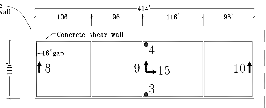
Basement Plan
