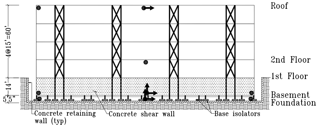
W/E Elevation
