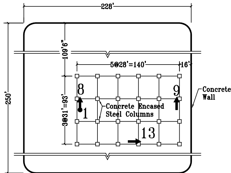
Basement Plan
