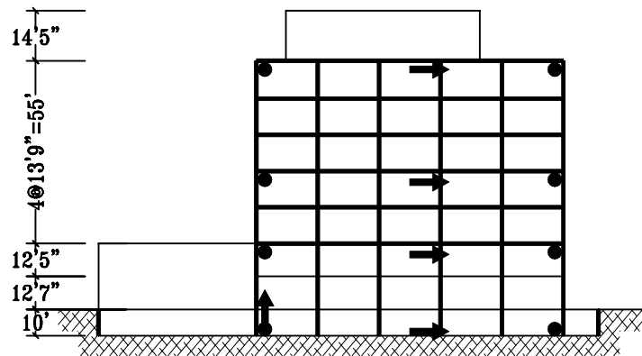
E/W Elevation
