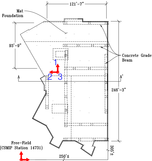
Foundation/Ground Floor
