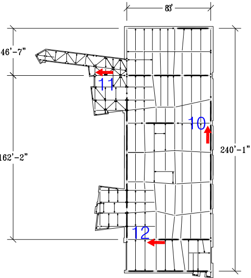
Third Floor
