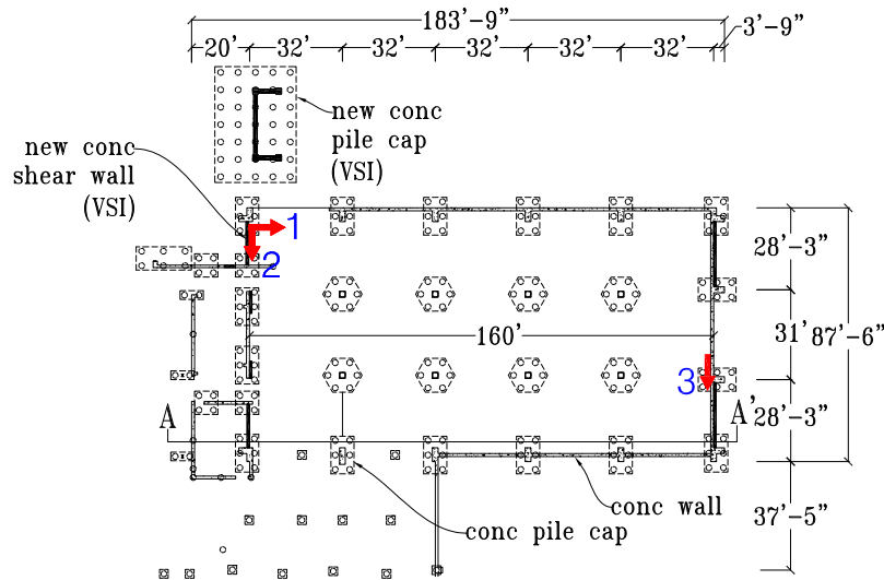
Basement/Foundation Plan
