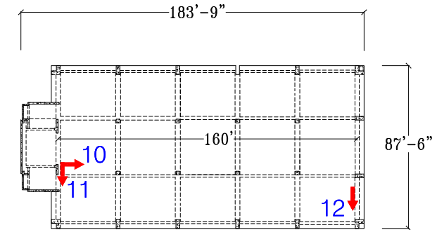
Roof Plan
