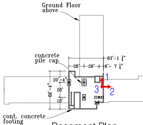
Basement Plan
