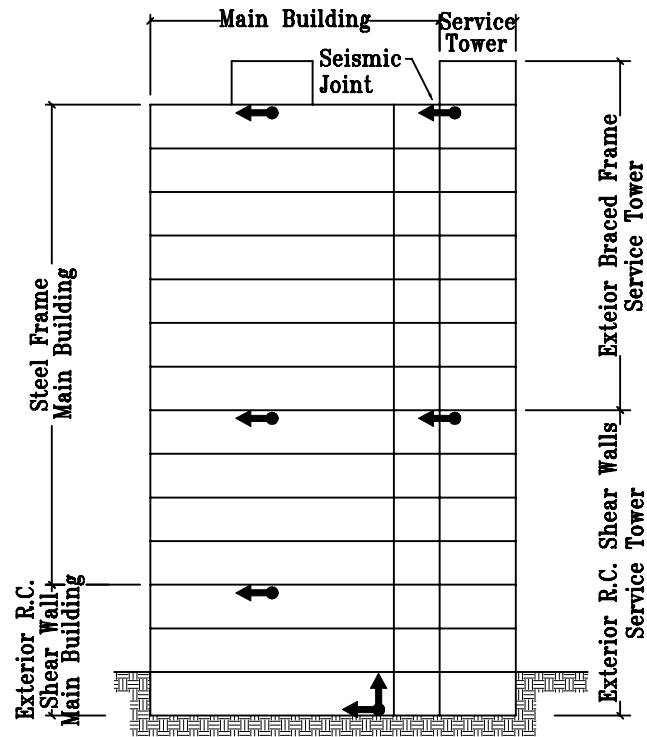
E/W Section
