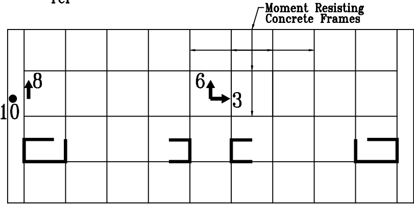
2nd Floor Plan
