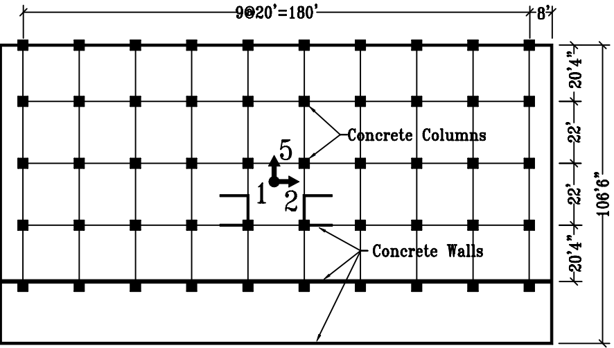
Basement Plan
