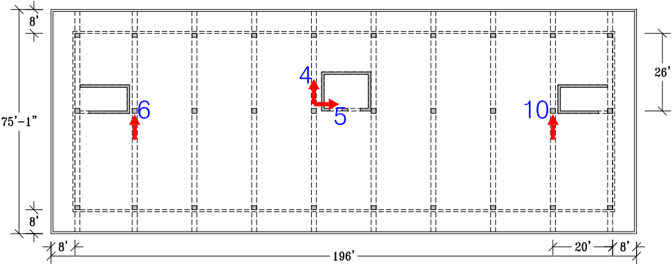
Roof Plan
