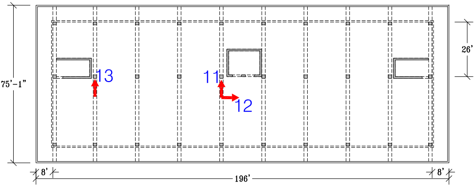
4th Floor Plan
