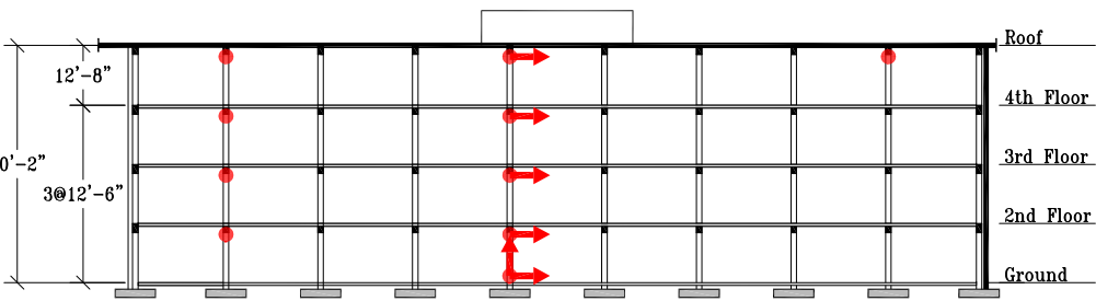
W/E Elevation
