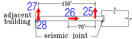
Level 3 Bridge Plan
