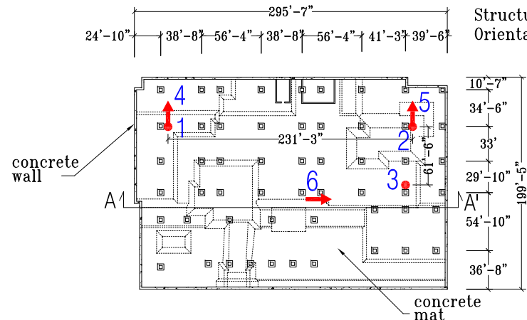
Level B2 Plan
