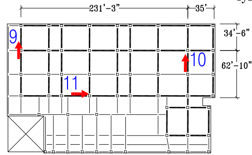
Level 4 Plan
