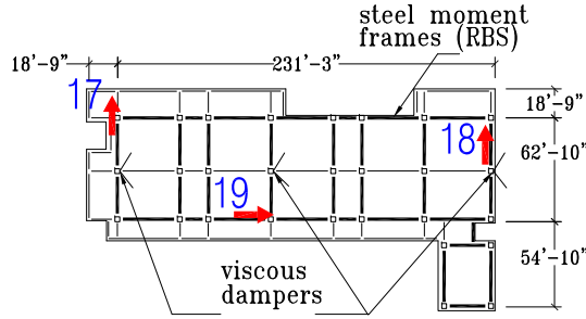
Level 17 Plan
