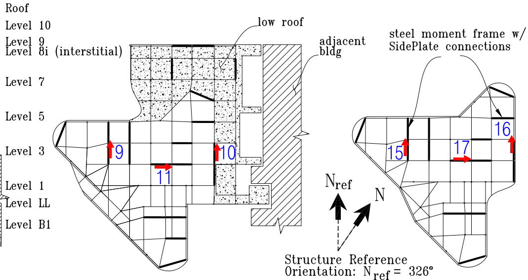
Level 3 Plan
