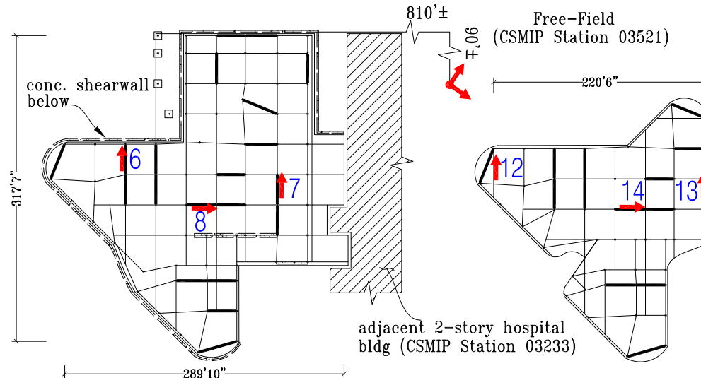
Level 1 Plan
