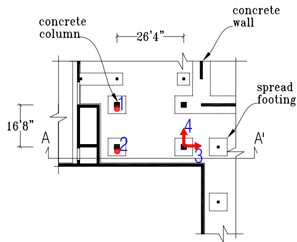
Basement Plan
