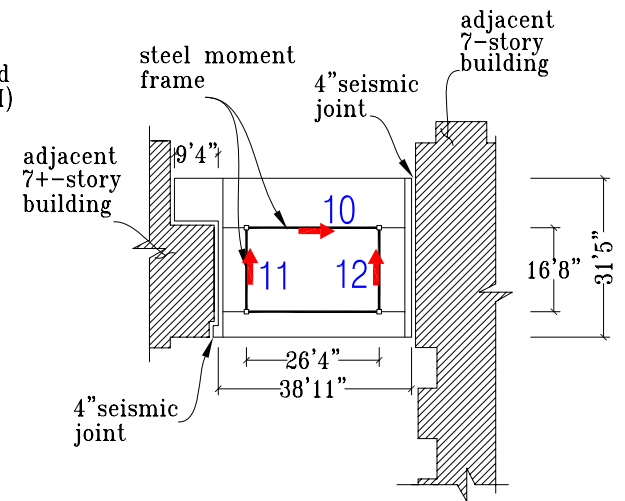
Roof Plan
