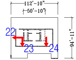
Lower Roof Plan
