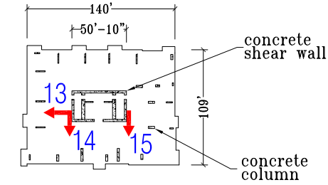
Level 14 Plan
